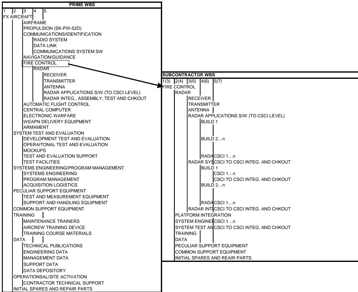
FIGURE 3-2: Relationship of Contract WBS to Subcontract WBS
